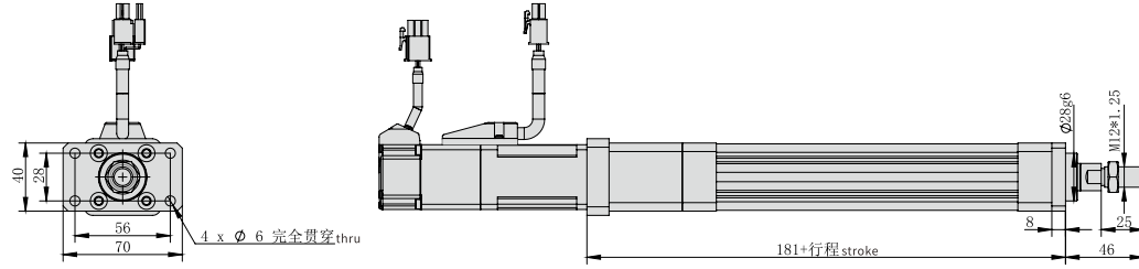
M 电机外置直连 Motor external direct connection
