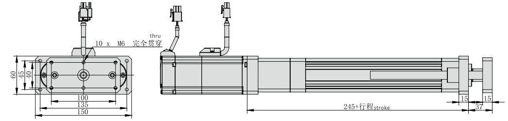
M 电机外置直连 Motor external direct connection 单位:Unit: mm
