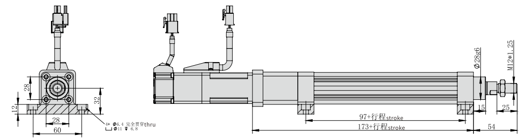
M 电机外置直连 Motor external direct connection
