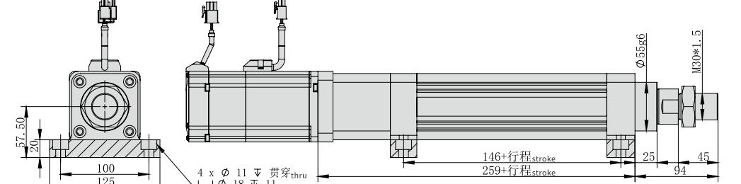
M 电机外置直连 Motor external direct connection 单位:Unit: mm
