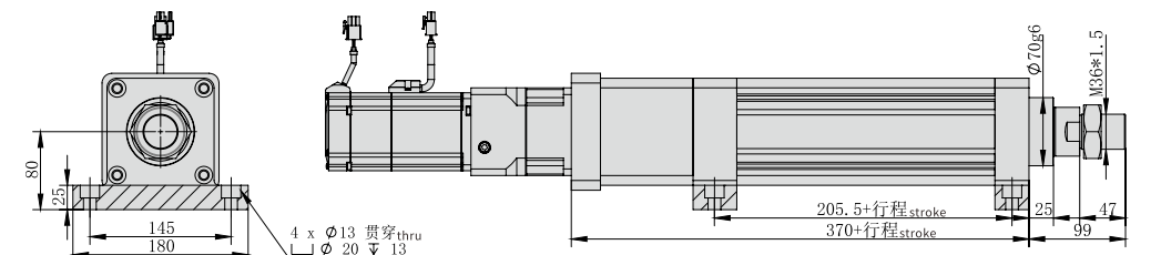
M 电机外置直连 Motor external direct connection
