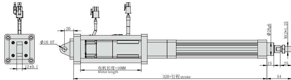
M 电机外置直连 Motor external direct connection
