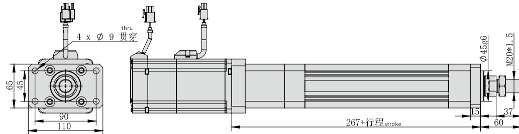
M 电机外置直连 Motor external direct connection 单位:Unit: mm
